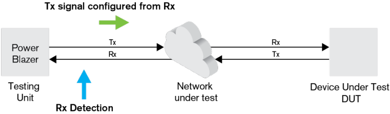
Figure 73. Automatic identification and configuration of tested frames
