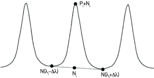
Figure 98. IEC 61280-2-9 method for measuring OSNR.
