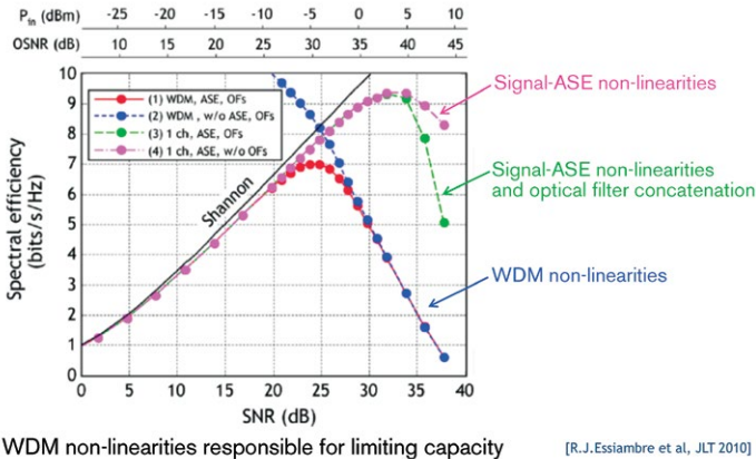
WDM non-linearities responsible for limiting capacity
