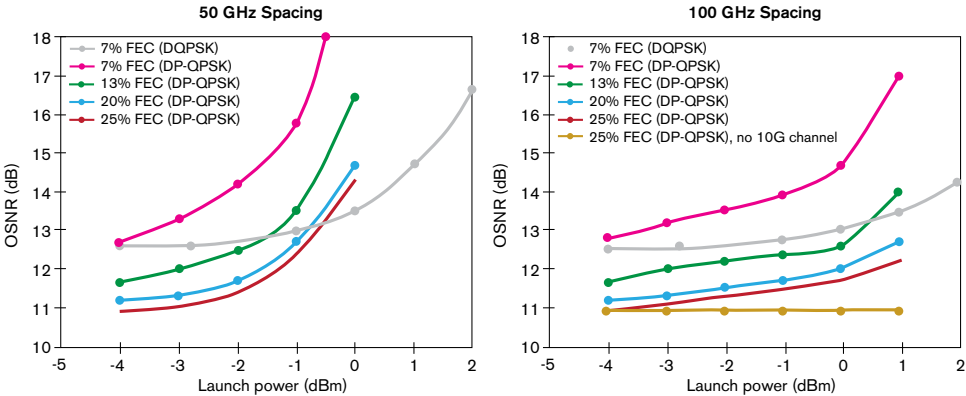
Figure 88. Relationship between OSNR and launch power.
