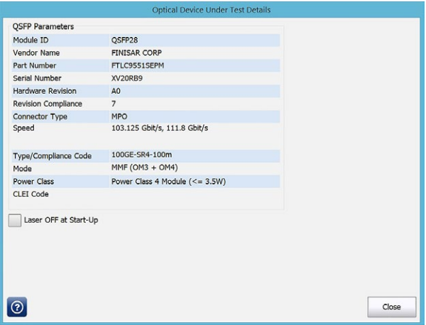
Figure 30. The QSFP details dialogue box.
