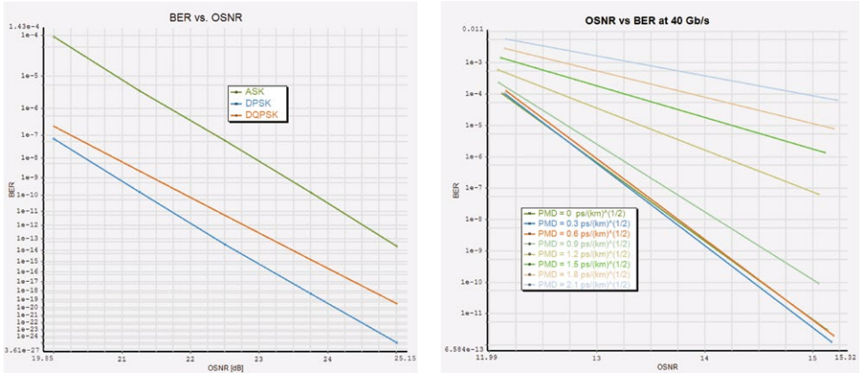
Figure 97. Relationship between OSNR and BER: a higher OSNR means a lower BER.
