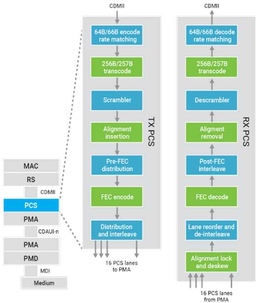
Figure 10. PCS layer
