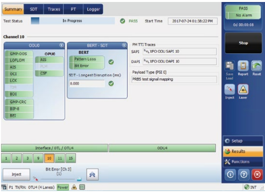
Figure 78. OTN summary page
