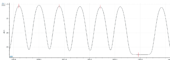
Figure 107. Trace with channel number seven turned off, ready for Pol-Mux OSNR calculation with the commissioning assistant.
