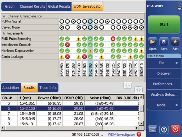
Figure 87. An example of non-linear depolarization in WDM Investigator.
