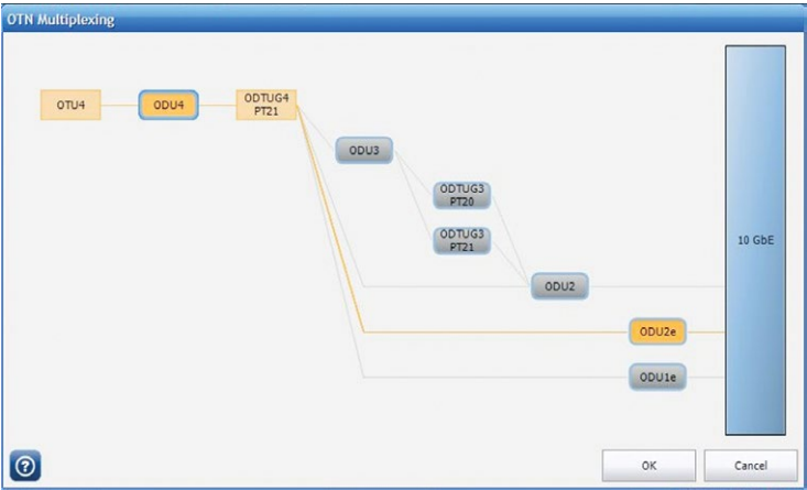
Figure 54. Mapping 10GE to ODU2e, and to OTU4.
