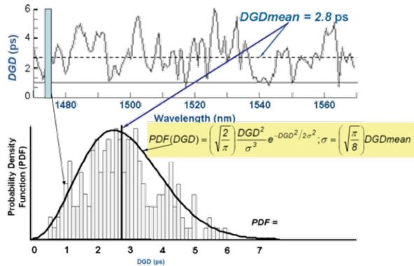
Figure 93. Relationship between PMD and instantaneous DGD.
