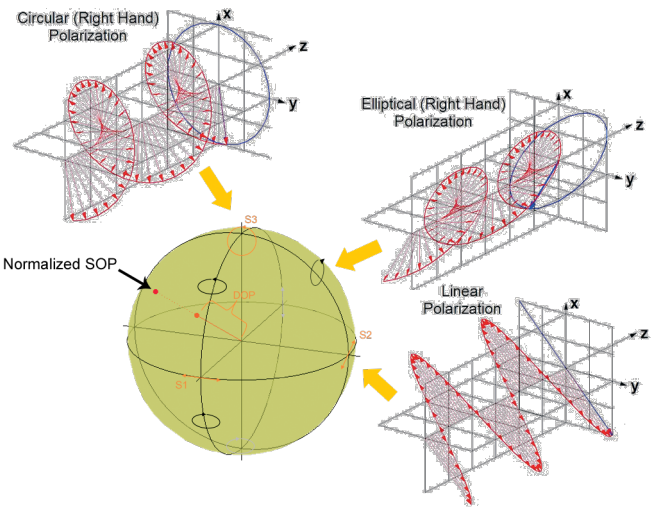
Figure 95. Poincaré sphere showing different SOPs.
