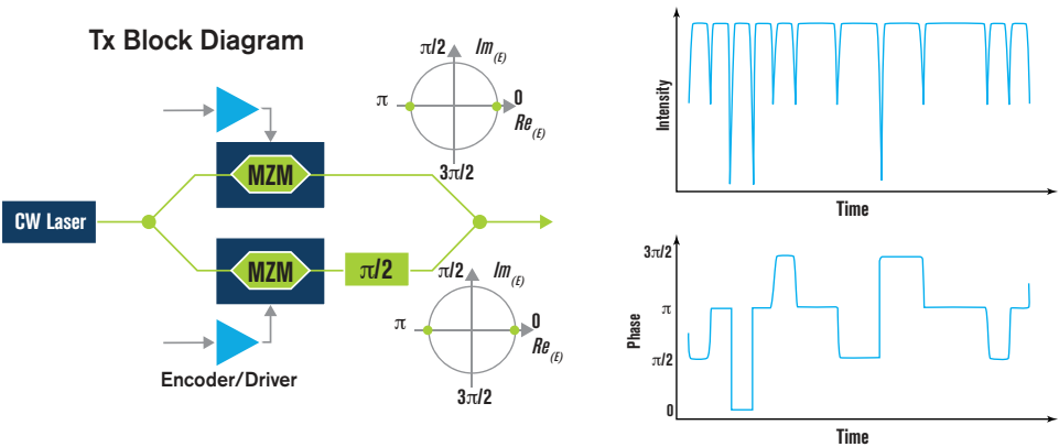
Figure 15. Block diagram of a DQPSK transmitter; intensity and phase diagrams of DQPSK transmitters.
