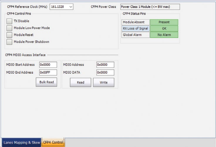
Figure 22. CFP4 status and MDIO access interface.
