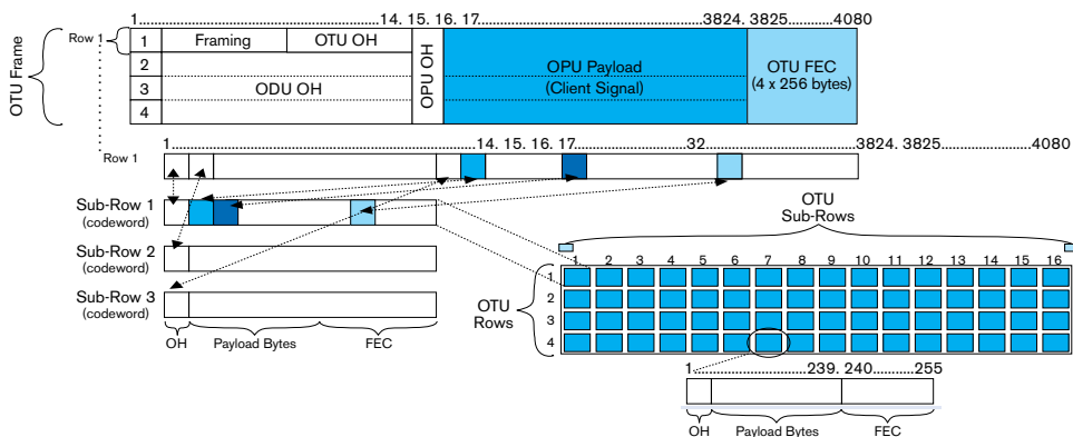
Figure 37. FEC interleaving in OTN.
