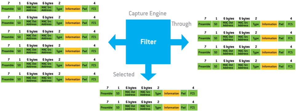
Figure 125. Traffic filtering mechanism.
