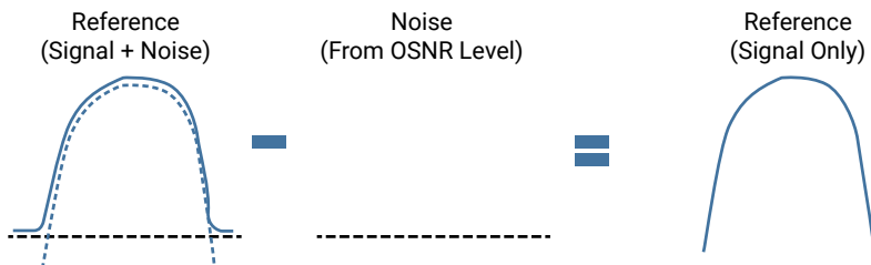
Figure 112. Computing a noise-free reference
