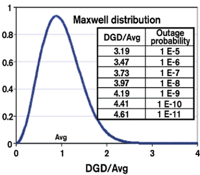
Figure 94. DGD vs. PMD Maxwellian distribution.
