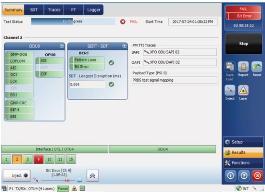
Figure 79. Status of every channel in the test configuration is color coded
