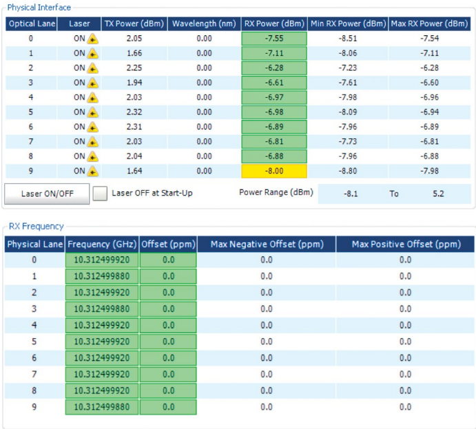
Figure 21. The EXFO's 88000 Power Blazer product family integrates a number of physical-layer diagnosis tools. The first picture shows the Rx power level of each optical lane. The second screenshot shows the frequency offset for each physical lane.
