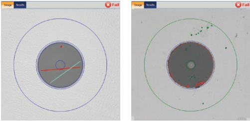
Figure 115. Endface scratches (left) and clad breakage (right).
