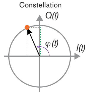
Figure 16. Constellation diagram.
