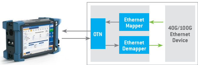
Figure 56. EXFO's 40G/100G portable solution.
