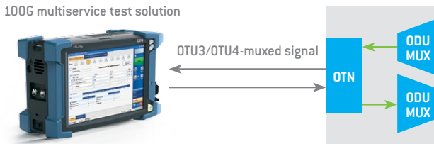
Figure 41. ODU-multiplexing test configuration.
