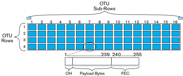
Figure 36. OTN rows and subrows.
