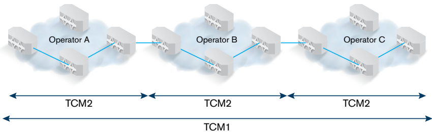
Figure 65. TCM allocation.
