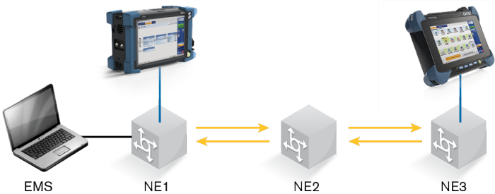
Figure 132. Test setup for quality-of-service verification.
