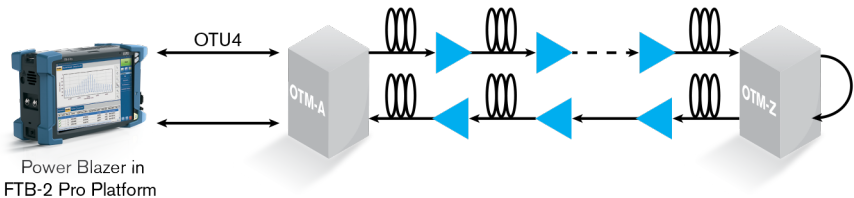
Figure 117. OTN long-term BER testing configuration
