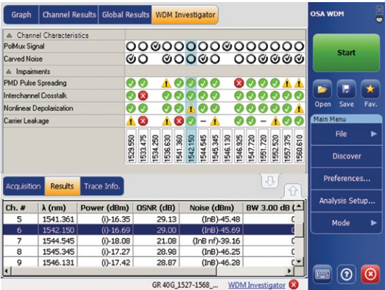
Figure 96. Example of PMD pulse spreading in WDM Investigator.
