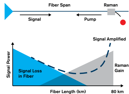
Figure 91. Counter-propagating Raman amplification.
