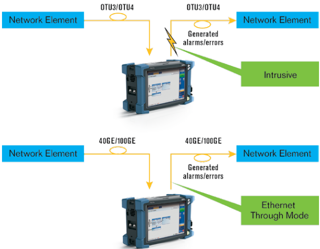
Figure 66. Through mode test configuration.
