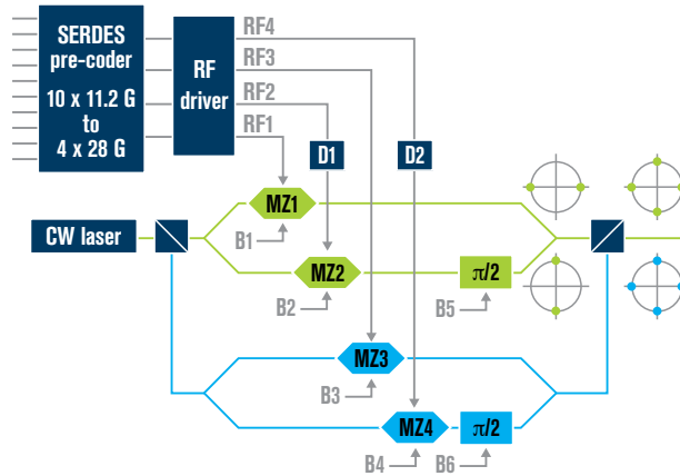
Figure 17. Block diagram of a DP-QPSK transmitter.
