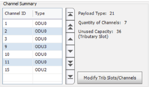
Figure 74. Summary of ODU container types
