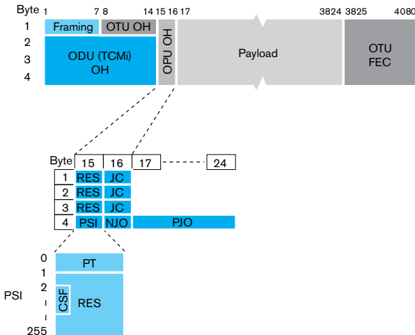
Figure 34. OPU overhead and structure.
