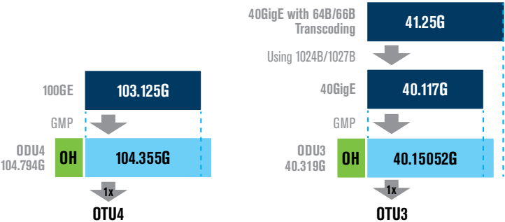
Figure 55. 40G/100G Ethernet mapped into OPU3/OPU4.
