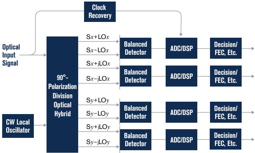
Figure 18. Components of a real-time electrical-sampling optical modulation analyzer.
