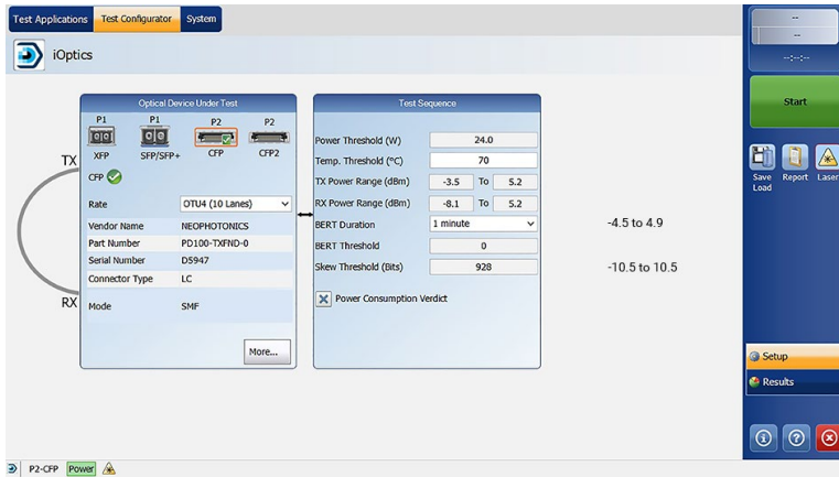
Figure 31. The iOptics test configuration page.
