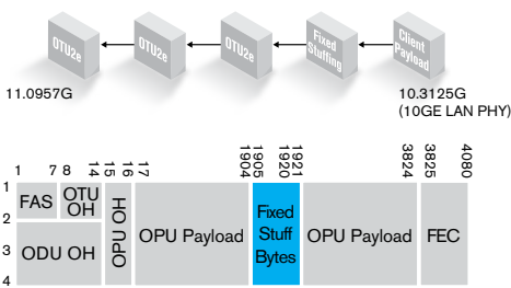
Figure 52. OTU2e with fixed stuff bytes.
