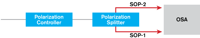
Figure 105. In-band OSNR setup.
