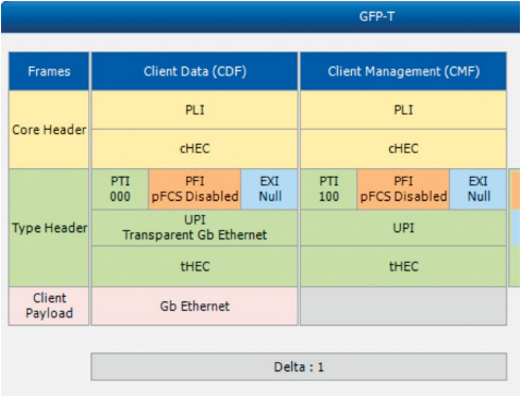
Figure 43. GFP-T overhead-byte analysis interface on EXFO's FTBx-88200NGE OTN analyzer.
