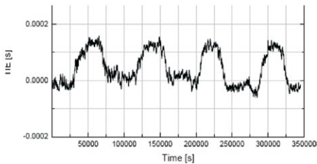
Figure 135. TIE test result.
