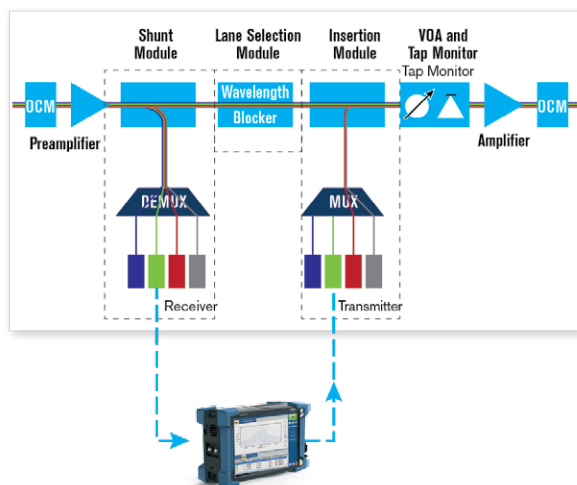
Figure 59. ROADMs-based network SDT measurement.
