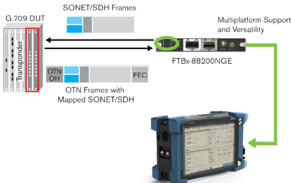
Figure 42. Client signal mapping test configuration: both the transmitting and receiving ports require the decoupling mode.
