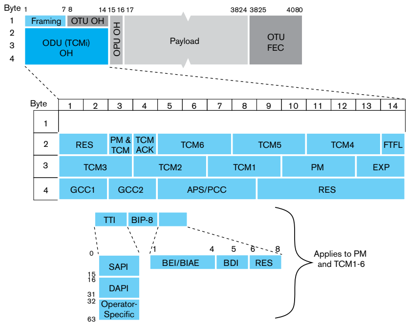
Figure 33. ODU overhead and structure.
