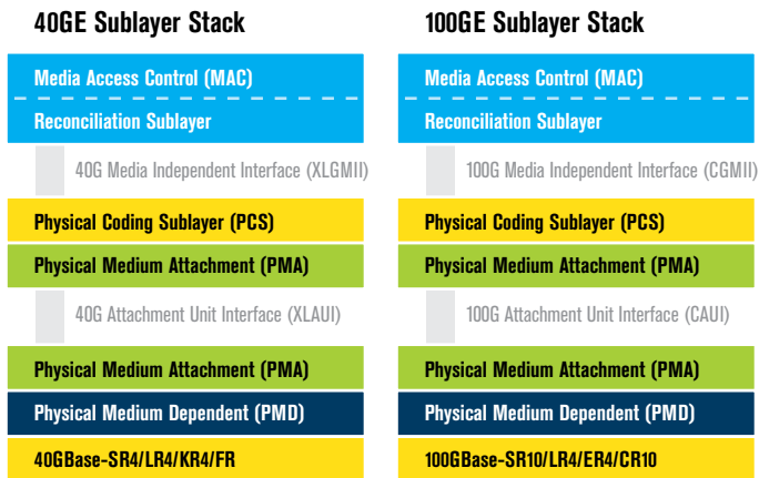
Figure 19. IEEE model with CAUI.
