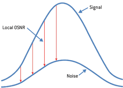
Figure 102. OSNR definition from IEC 61282-12 standard.
