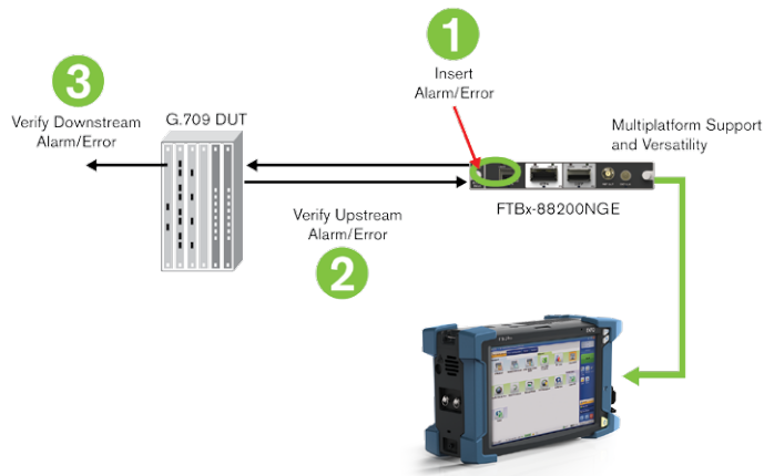
Figure 39. Connection diagram of response test using EXFO's FTB-2 Pro.
