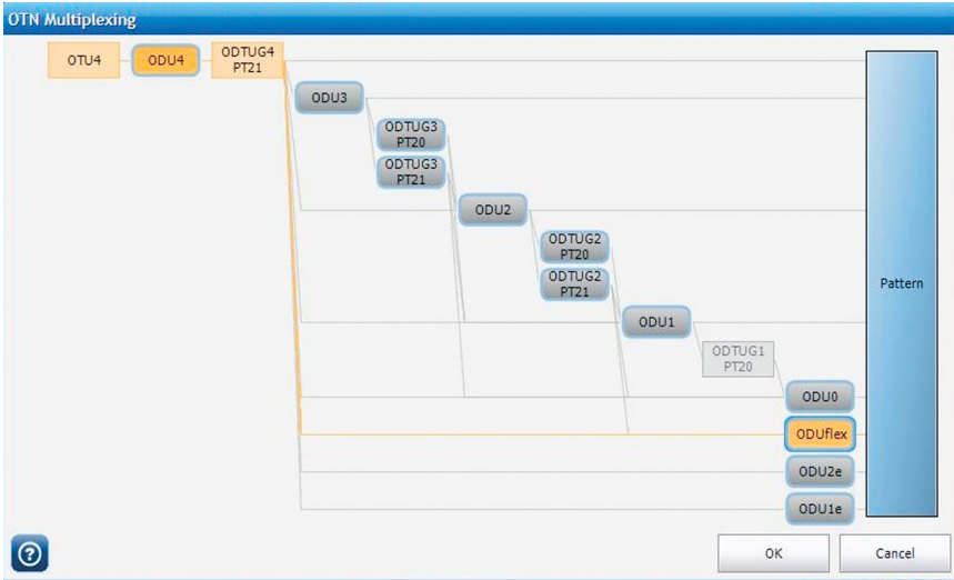
Figure 45. Mapping of Pattern-ODUFlex-ODU4.
