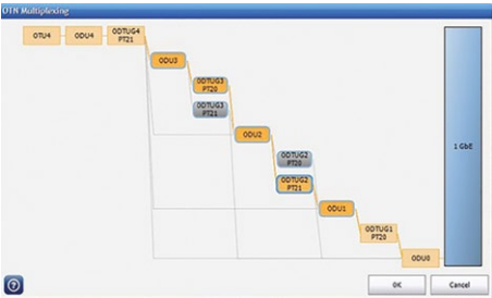
Figure 48. GE-ODU0-ODU1-ODU2-ODU3-ODU4 signal structure interface.
