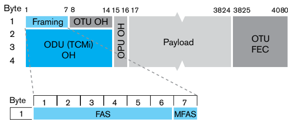
Figure 32. G.709 frame alignment.
