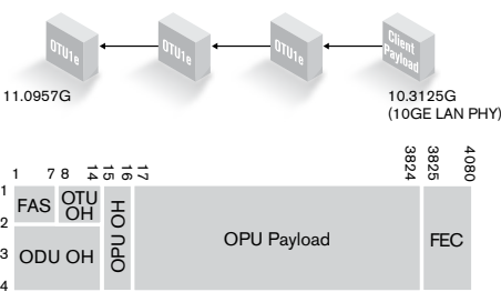
Figure 53. OTU1e without fixed stuff bytes.
