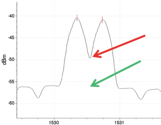
Figure 100. Noise level of 40G channels. Red arrow: noise level using the IEC method. Green arrow: real noise level.
