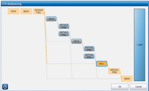
Figure 49. GE-ODU0-ODU1-ODU4 signal structure interface.
