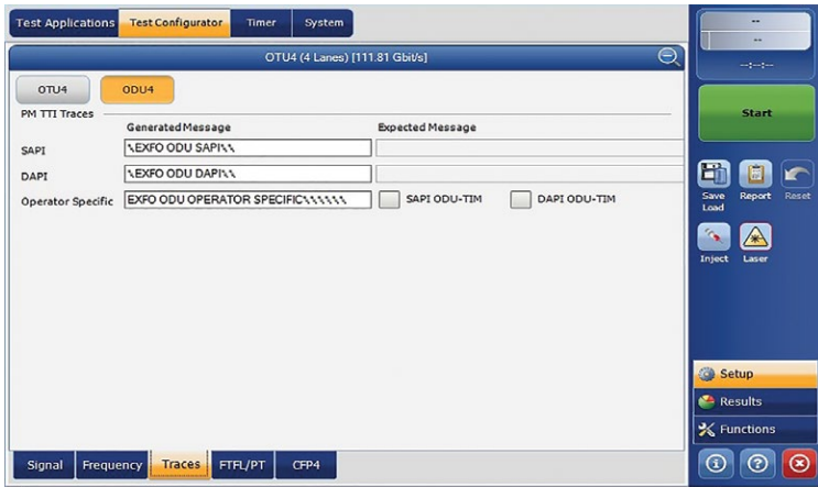
Figure 116. TTI SAPI/DAPI/operator information test using the FTB-88100NGE Power Blazer.
