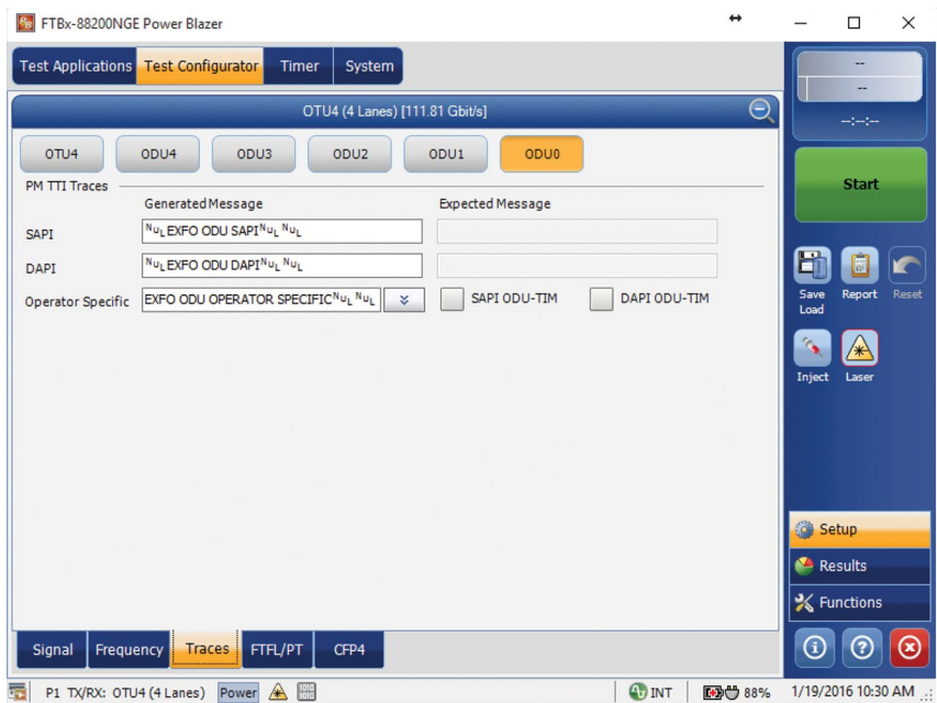
Figure 64. Testing of TTI SAPI/DAPI/operator information using the FTBx-88200NGE Power Blazer.
