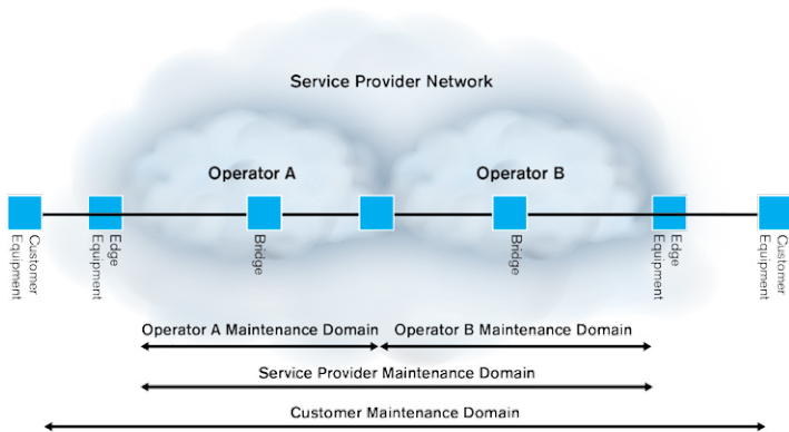
Figure 127. Hierarchical maintenance domain.
