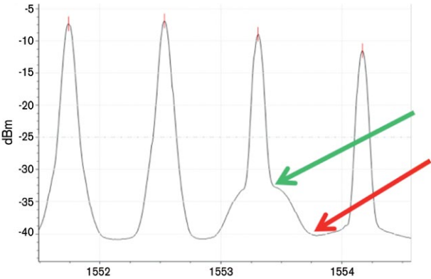
Figure 99. Noise level of a filtered channel. Red arrow: noise level using the IEC method. Green arrow: real noise level.
