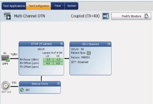
Figure 70. Configuration of 80 ODU0 channels on an ODU4
