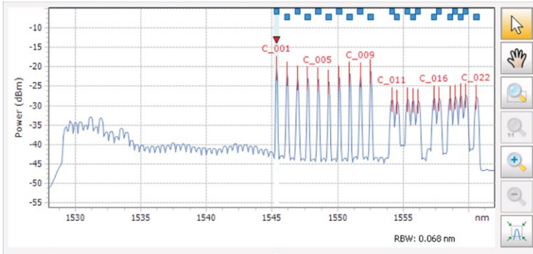
Figure 101. Spectrum with 10G channels in a ROADM network and 40G channels.
