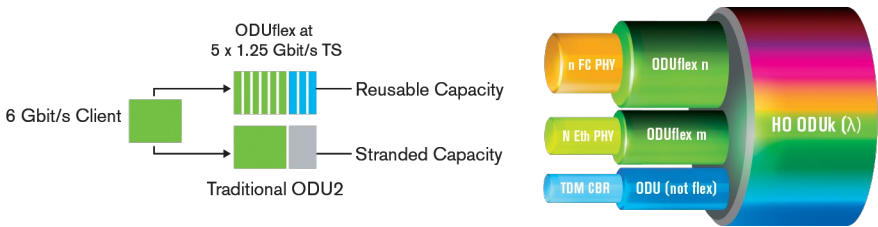
Figure 44. Reusable capacity via ODUflex.
