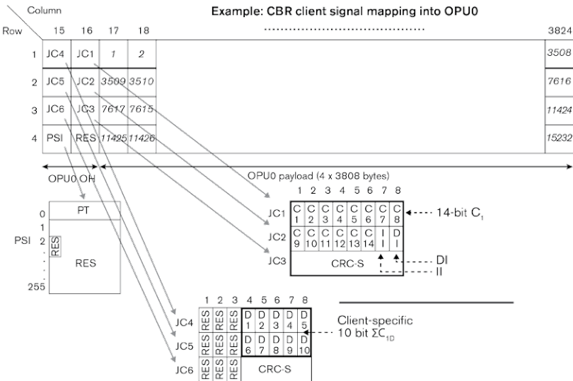
Figure 47. GMP justification-control bytes.
