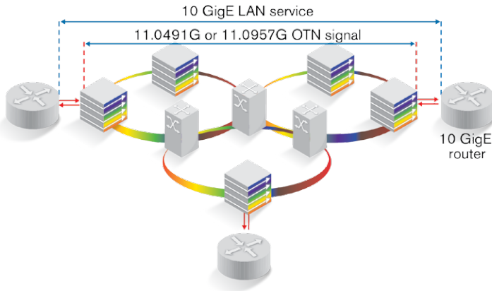
Figure 50. Application scenario of overclocked OTN.
