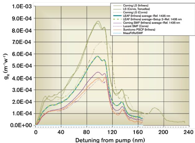
Figure 92. Raman gain distribution for various commercially available fibers.
