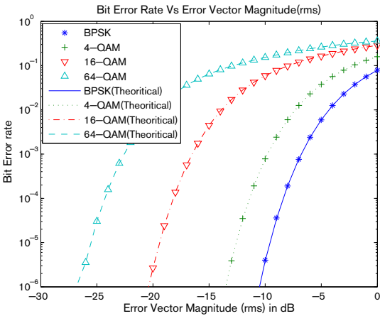
Figure 113. BER vs. EVM relationship for different modulation formats.
