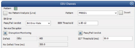
Figure 76. User provided SDT threshold
