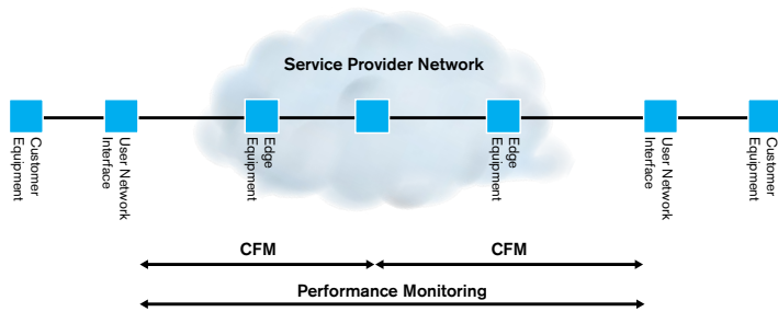
Figure 126. Customer maintenance domain.
