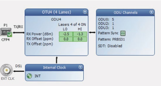
Figure 71. Sample test configuration
