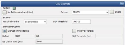
Figure 75. BER testing
